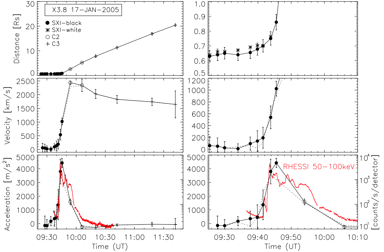
Fig. 2.— Event of 2005 January 17. From top to bottom: Distance-time profile d(t) , velocity v(t) and acceleration a(t) of the CME as observed by different instruments (different plot symbols specified in the legend). In the bottom panel, we plot also the RHESSI 50–100 keV HXR flux of the associated flare. The left panels show the full CME height range covered by the LASCO FoV, i.e. up to 30 R_\odot . The right panels zoom into the early acceleration phase of the CME as observed against the solar disk in SXI. The solid curves connects the “black” features measured in the SXI running ratio images and subsequent LASCO measurements, the dashed curves refer to the “white” features.
