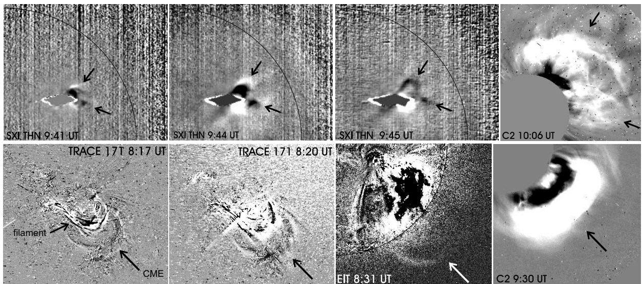
Fig. 1.— Top: 2005 January 17 CME. Sequence of three SXI running ratio images and one LASCO C2 running difference image. Bottom: 2006 July 6 CME. Sequence of two TRACE 171 Å, one EIT 195 Å and one LASCO C2 running difference images.
