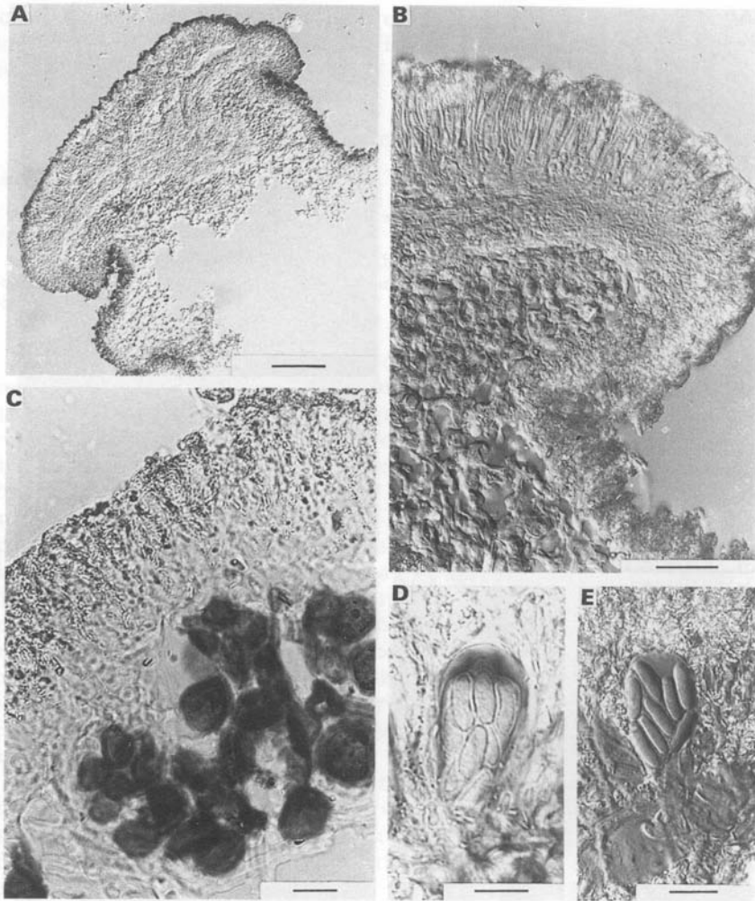
FIG. 2. Vertical section through ascocarp and thallus of Lecanora somervellii . A, Apothecium. B, Margin of apothecium. C, 'True cortex', lacking algal cell walls (in chlor-zinc-iodine). D, Mature ascus (in Lugol's iodine), with broad 'chambre oculaire' and 'masse axiale'. E, Ascospores. Scales: A = 100 \mu m; B = 50 \mu m; C-E = 10 \mu m.
