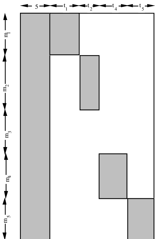
Figure 1: Matrix A
