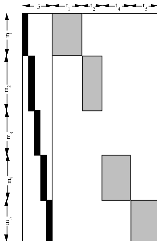
Figure 2: Matrix B
